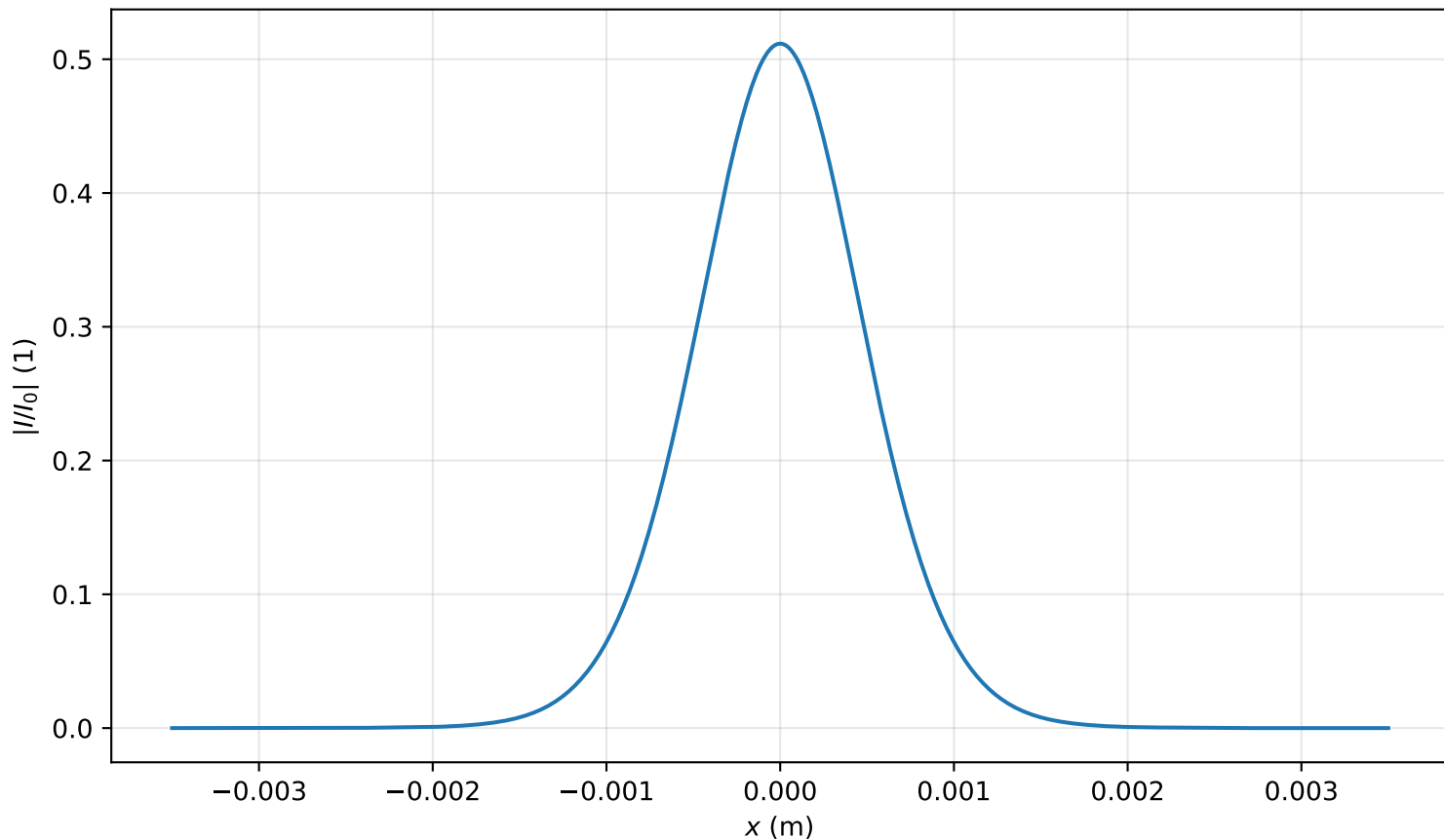
Intensity profile I(x, y = 0, z = 2.866m)/I_0 , P_{in}=0.4P_{cr} , artificial time
